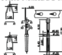
0.76 Crimp Pin Female PART No.:HDBC-FT-L
