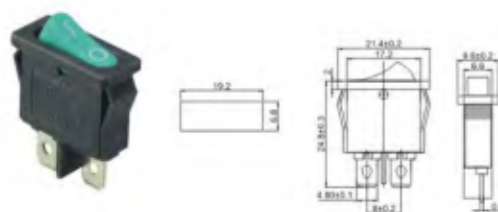
A-TOP1-12-101 ON-OFF
