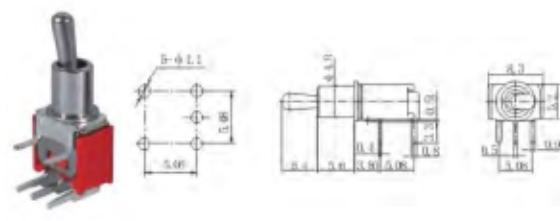
BTS-102-2C3 ON-ON BTS-103-2C3 ON-OFF-ON SPDT 3P
