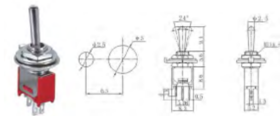
BTS-103-2A1 ON-OFF-ON SPDT 3P
