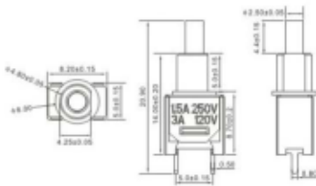
T-TOP-101 OFF-(ON) 1.5A 250VAC
