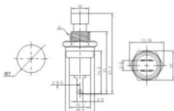
T-TOP-105 OFF-(ON) T-TOP-105C ON-(OFF) 0.5A 250VAC
