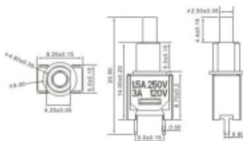
T-TOP-101 OFF-(ON) 1.5A 250VAC
