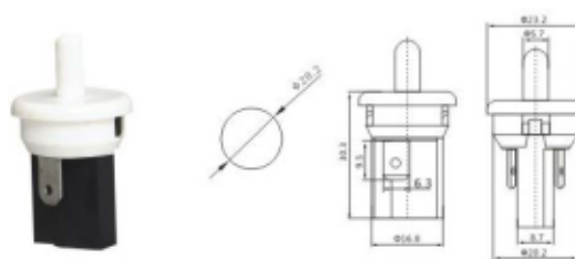
T-TOP-35C ON-(OFF) 3A 125VAC; 1A 250VAC
