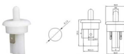
T-TOP-35B OFF-(ON) 3A 125VAC; 1A 250VAC
