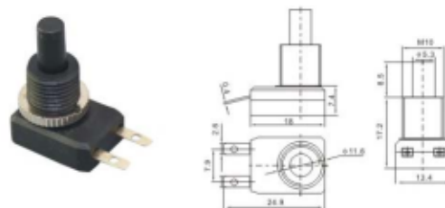
T-TOP-104 ON-OFF 1A 250VDC
