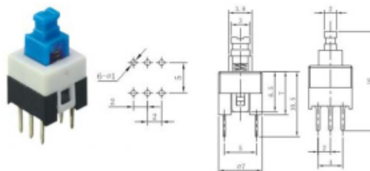
T-TOP-C7x7-A ON-ON T-TOP-C7x7-B ON-(ON)
