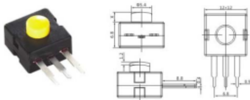
T-TOP-05 ON-ON-OFF 1A 30VDC
