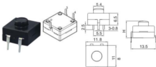
T-TOP-07-112-P3 ON-OFF T-TOP-07-213-P34 ON-ON-OFF
