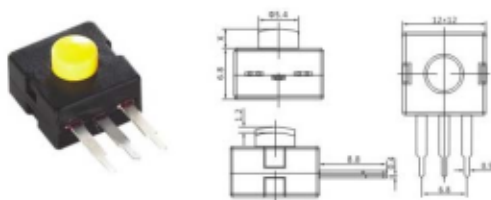
T-TOP-05 ON-ON-OFF 1A 30VDC
