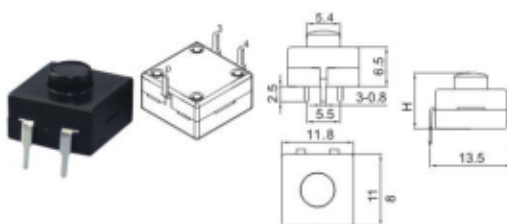
T-TOP-07-112-P3 ON-OFF T-TOP-07-213-P34 ON-ON-OFF
