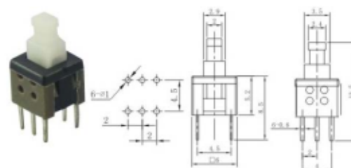
T-TOP-C6x6-A ON-ON T-TOP-C6x6-B ON-(ON)
