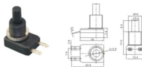
T-TOP-104 ON-OFF 1A 250VDC
