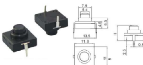
T-TOP-06 ON-OFF 1A 30VDC
