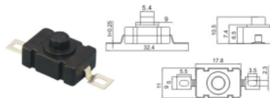
T-TOP-28 ON-OFF 1A 250VAC; 1A 30VDC
